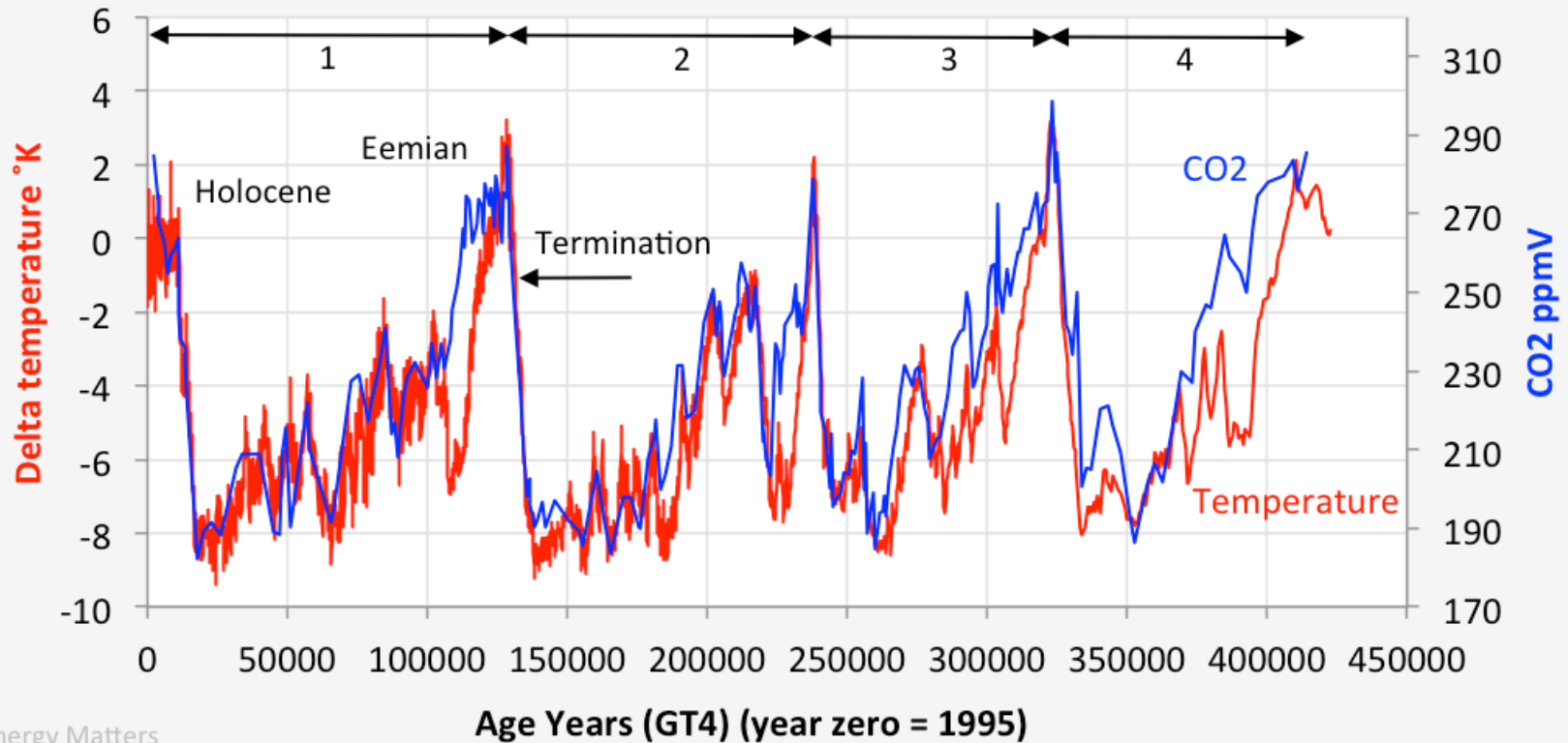
Vostok Ice Core: Temperature and CO 2
